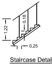
Staircase Detail
