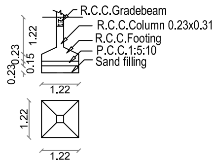
Foundation details-1
