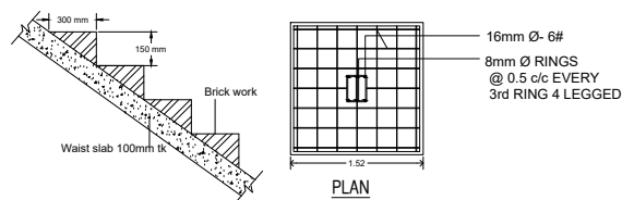
DETAIL OF STAIRCASE.
