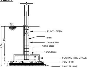
FOUNDATION & COLUMN DETAILS
