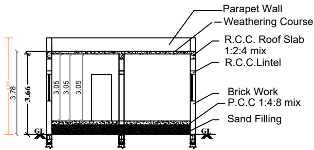
SECTION ON - SD
