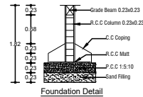
Foundation Detail
