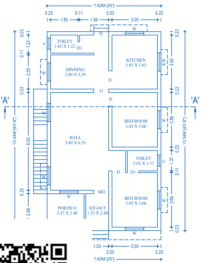
FLOOR PLAN
