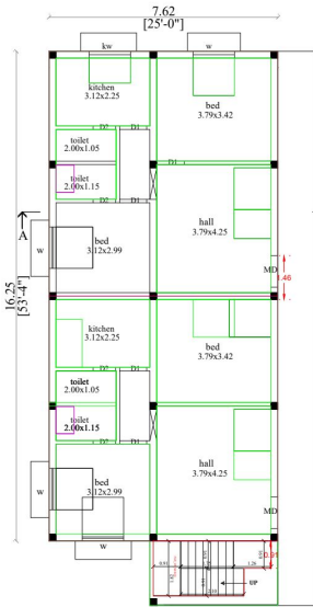
PRO., FIRST FLOOR PLAN
