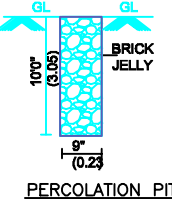
PERCOLATION PIT
