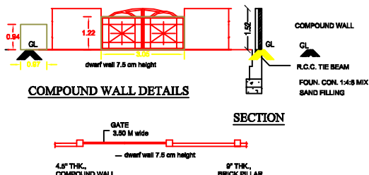
COMPOUND WALL PLAN
