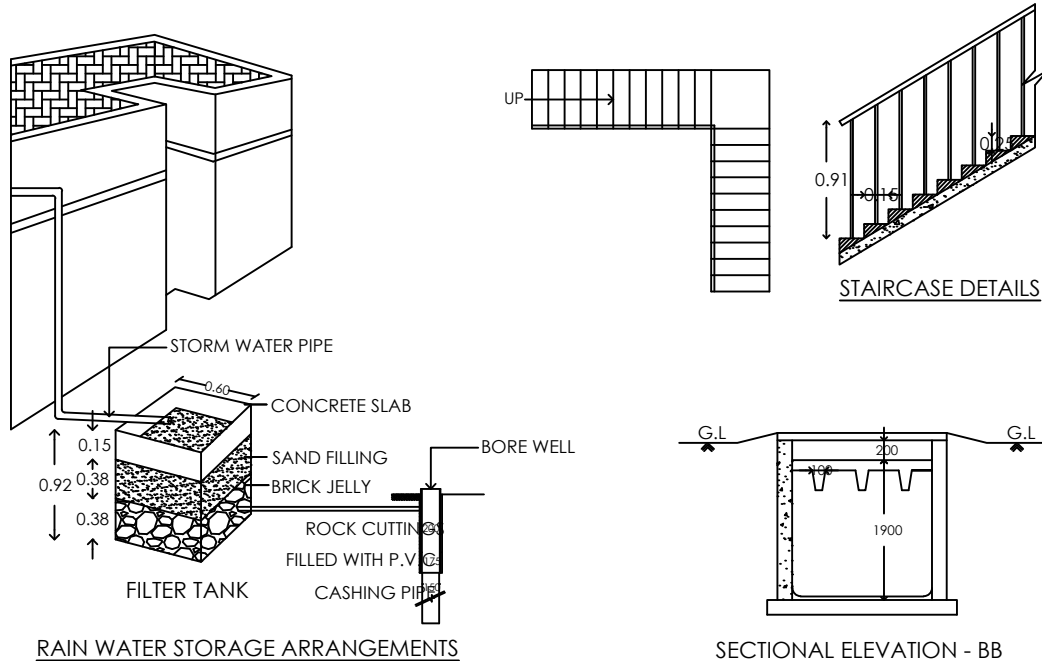
RAIN WATER STORAGE ARRANGEMENTS
