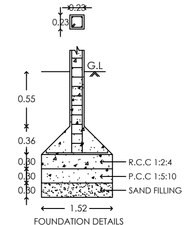
FOUNDATION DETAILS
