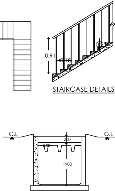
SECTIONAL ELEVATION - BB
