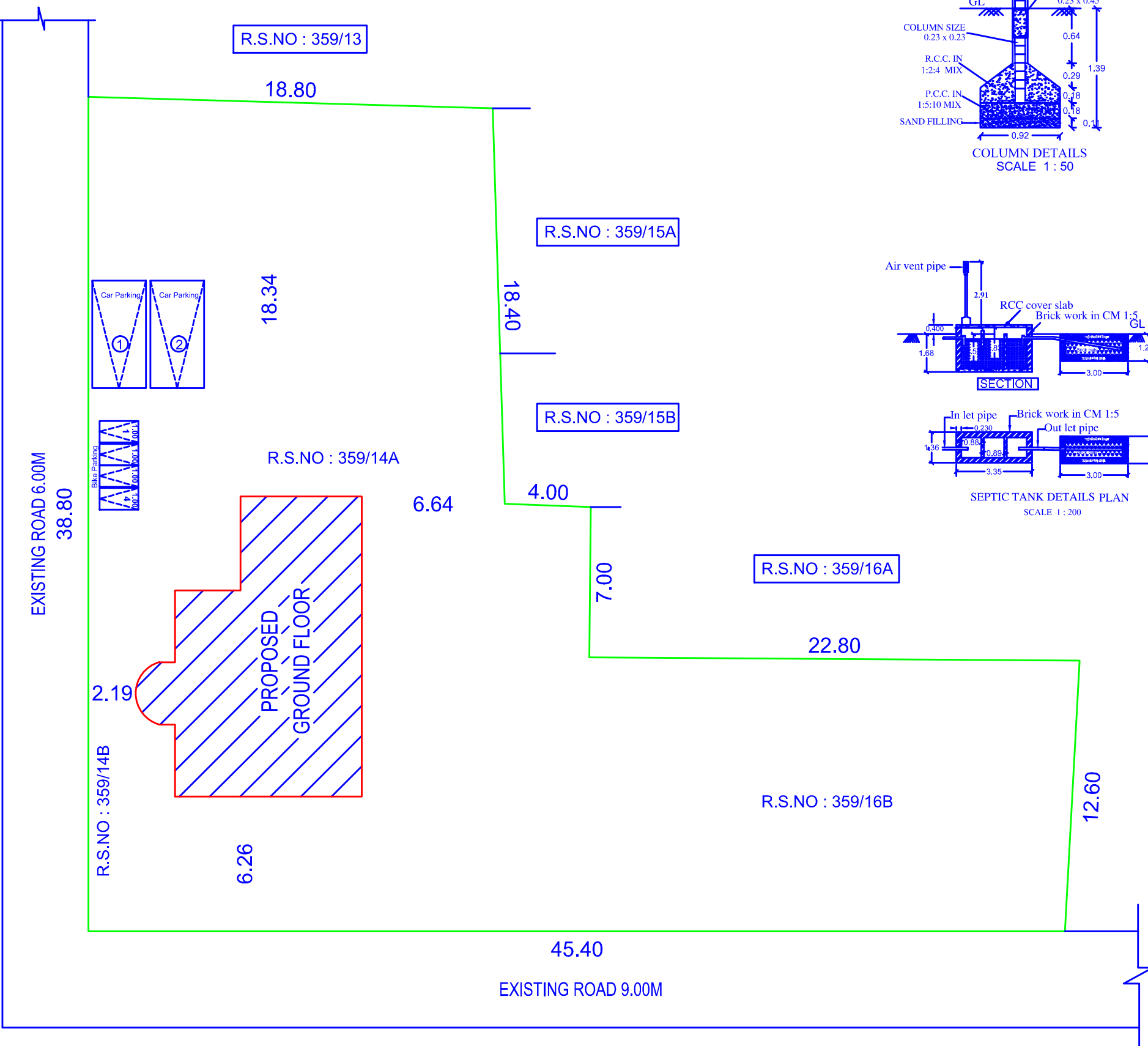
SITE PLAN
