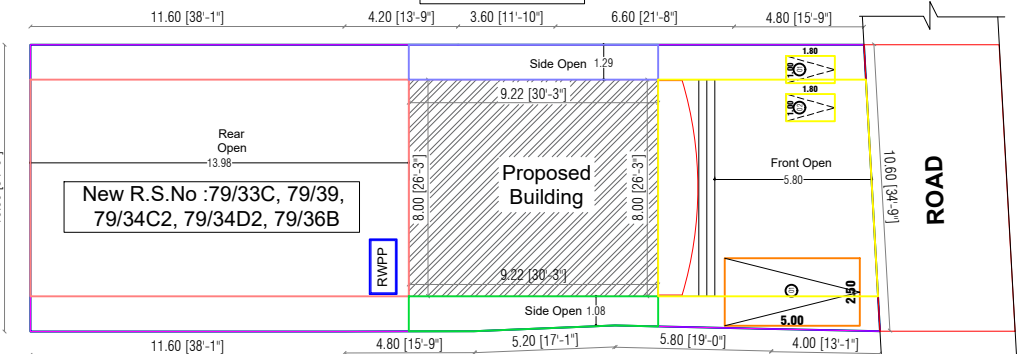
SITE PLAN
