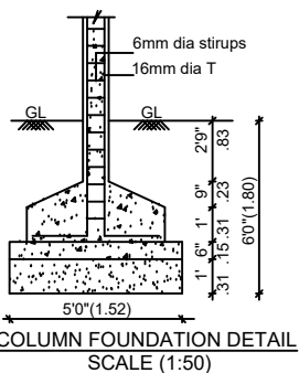
COLUMN FOUNDATION DETAIL SCALE (1:50)
