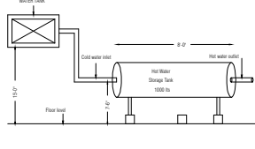
SOLAR WATER HEATER DETAILS (NOT TO SCALE)
