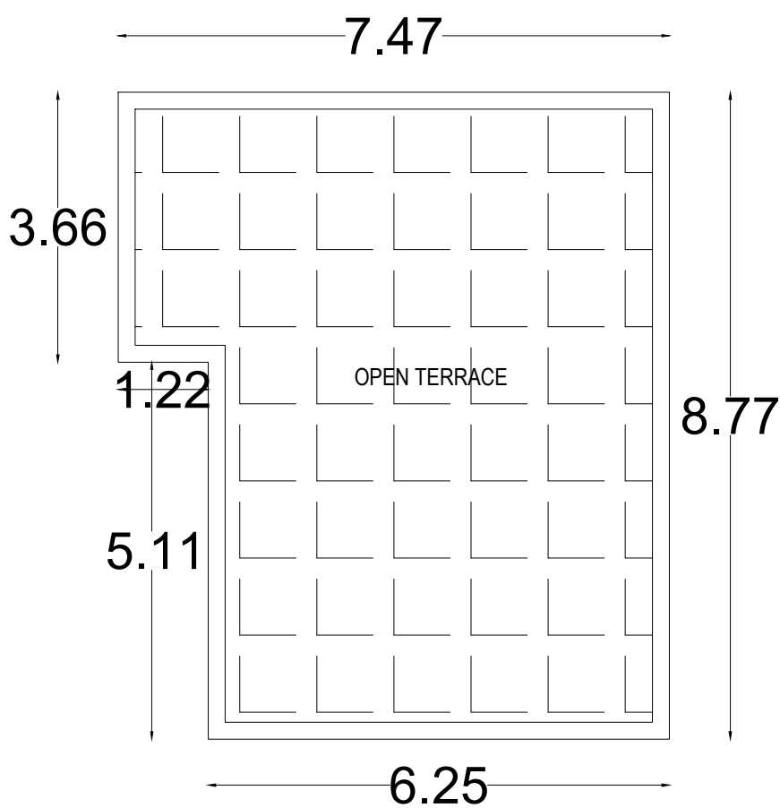
PRO. TERRACE FLOOR PLAN
