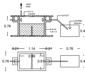
SEPTIC TANK & D-TRENCH DETAILS (NOT TO SCALE)
