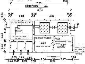
SEWAGE TREATMENT PLANT (S.T.P.) WASTE WATER FILTRATION BY RECIRCULATION SYSTEM G.O(MS) NO.138 DT:11.10.02
