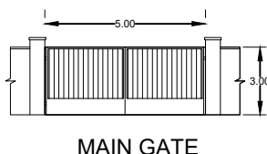
MAIN GATE
