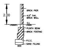
COMPOUND WALL
