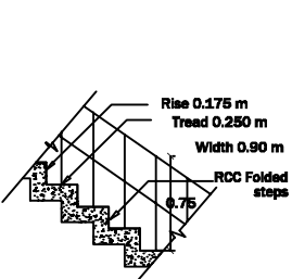
STAIRCASE DETAILS
