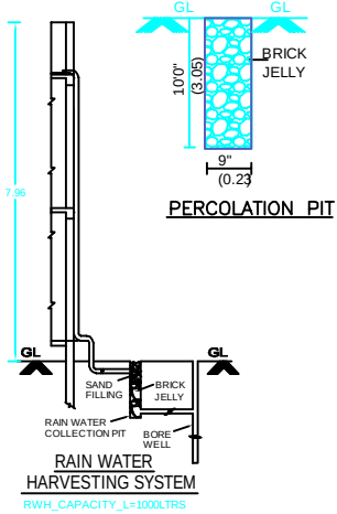
RAIN WATER HARVESTING SYSTEM
