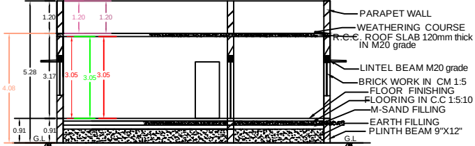
SECTION ON XX
