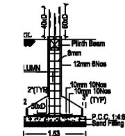
FOUNDATION DETAILS SCALE : 1:50
