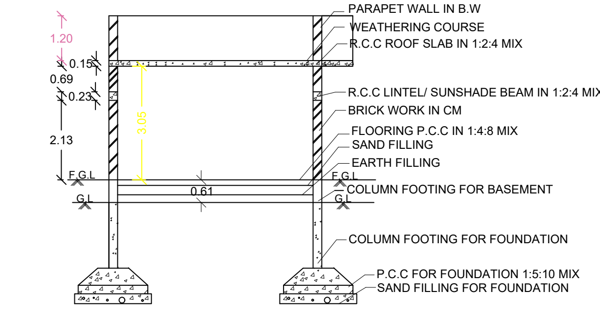
SECTION ON-AA1
