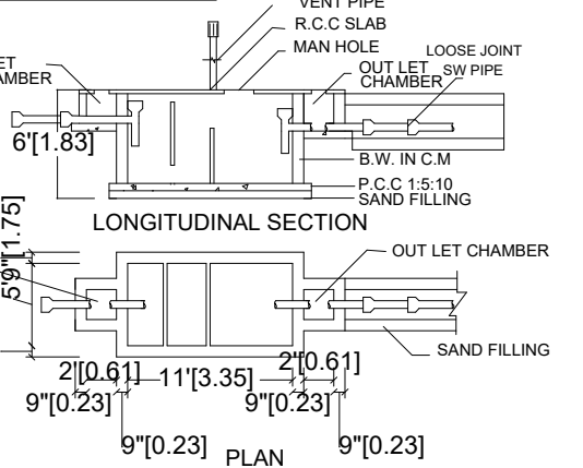
SEPTIC TANK:
