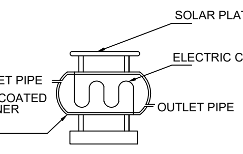
SOLAR SYSTEM
