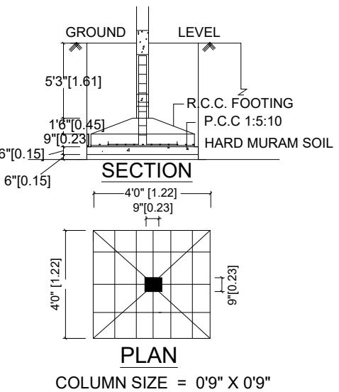
PLAN COLUMN SIZE = 0'9" X 0'9"
