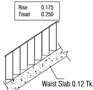
Staircase Details
