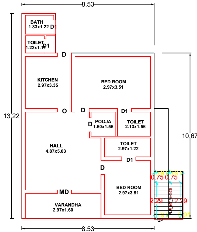
EXG.GROUND FLOOR PLAN
