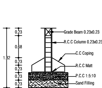
Foundation Detail
