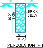
PERCOLATION PIT
