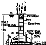
FOUNDATION DETAILS
