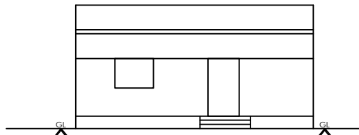
ELEVATION-AB
