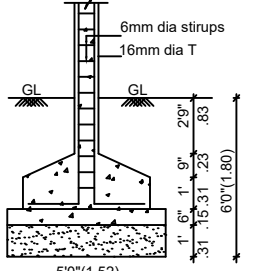
COLUMN FOUNDATION DETAIL
