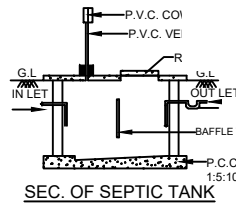
SEC. OF SEPTIC TANK
