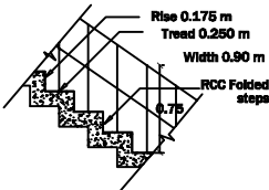
STAIRCASE DETAILS
