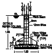
FOUNDATION DETAILS
