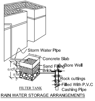
RAIN WATER STORAGE ARRANGEMENTS
