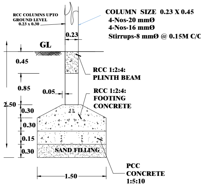
FOUNDATION DETAILS
