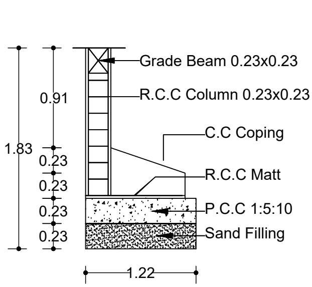
Foundation Details
