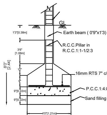
FOUNDATION DETAILS
