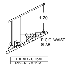
STAIRCASE DETAILS [ NTS ]
