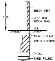
COMPOUND WALL
