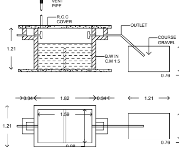
SEPTIC TANK & D-TRENCH DETAILS [ NOT TO SCALE ]
