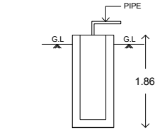
RWH_CAPACITY_L=5000LTRS DETAILS OF RAINWATER COLLECTION TANK
