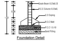
Foundation Detail
