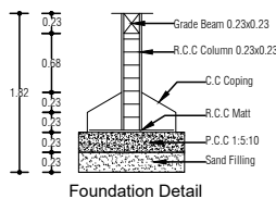
Foundation Detail
