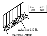
Staircase Details
