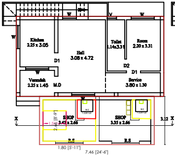
EXISTING GROUND FLOOR RESIDENTIAL BUILDING & PROPOSED GROUND FLOOR COMMERCIAL SHOP BUILDING PLAN
