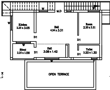
EXISTING FIRST FLOOR RESIDENTIAL BUILDING PLAN
