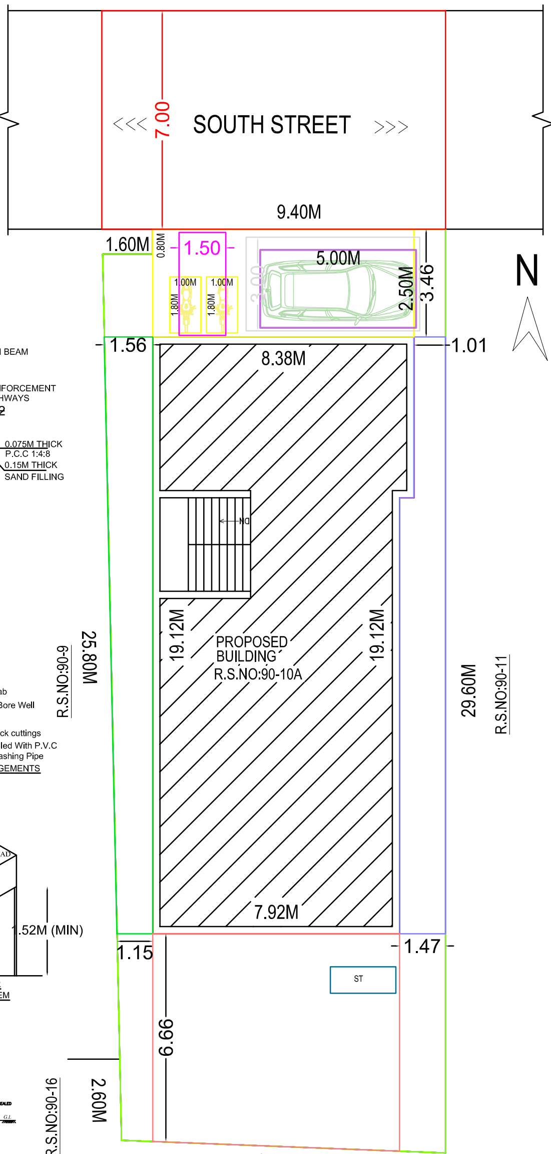
SITE PLAN
