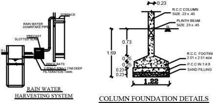
RAIN WATER HARVESTING SYSTEM
