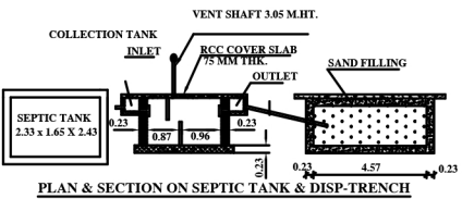
PLAN & SECTION ON SEPTIC TANK & DISP-TRENCH
