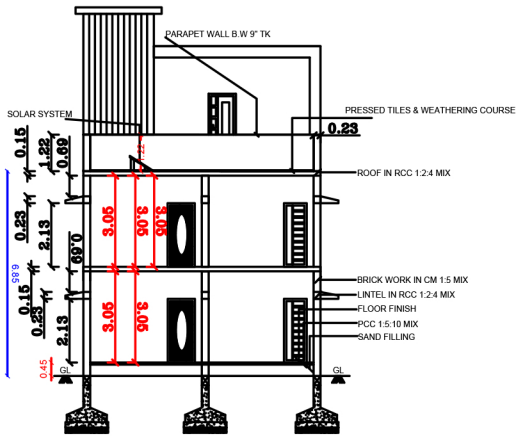
CROSS SECTION AB
