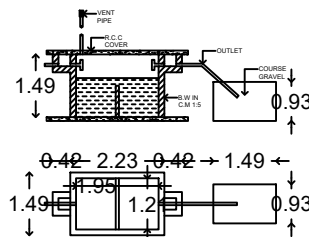
SEPTIC TANK & D-TRENCH DETAILS [NOT TO SCALE]
