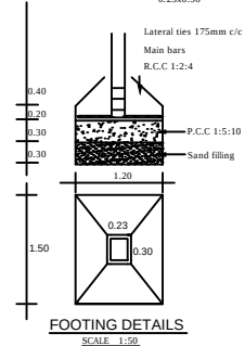
FOOTING DETAILS
