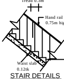
STAIR DETAILS
