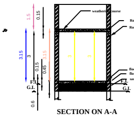
SECTION ON A-A
