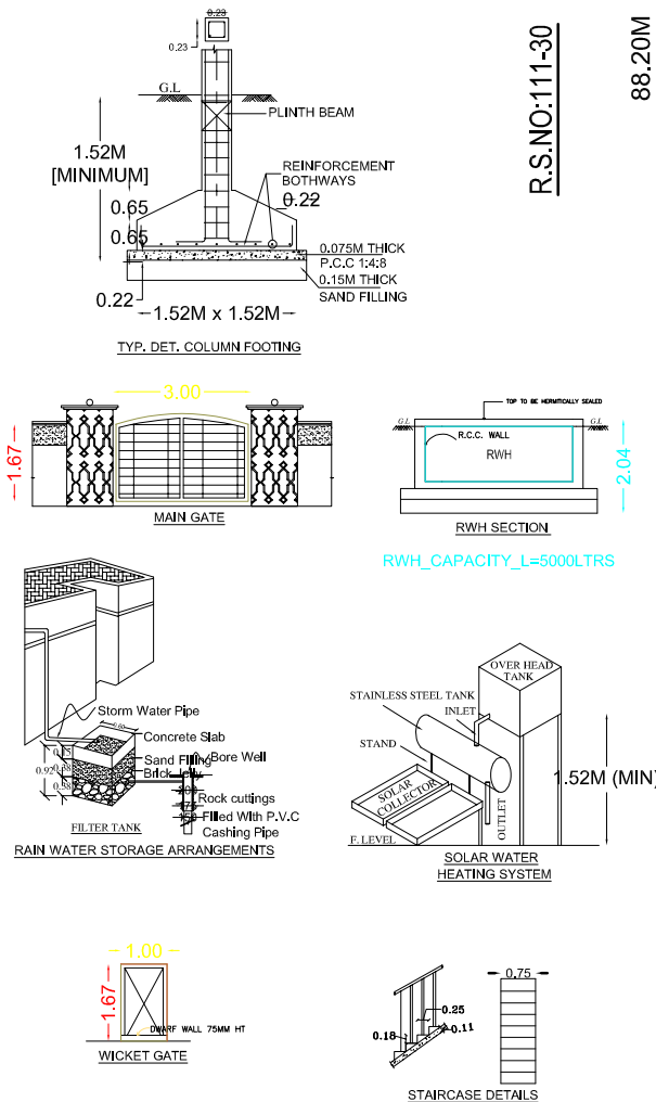
STAIRCASE DETAILS
