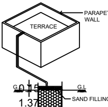
COLLECTION SUMP FOR HARVESTING FOR TERRACE
