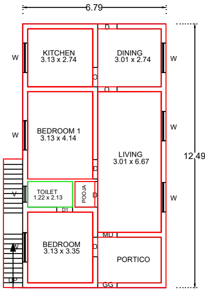
PRO. GROUND FLOOR PLAN
