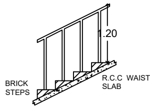
STAIRCASE DETAILS [ NTS ]
