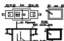
FOUNDATION DETAILS
