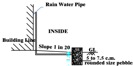
RAINWATER HARVESTING
