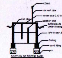
SECTION OF SEPTIC TANK
