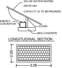
SOLAR SYSTEM
