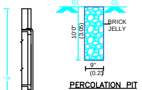
PERCOLATION PIT
