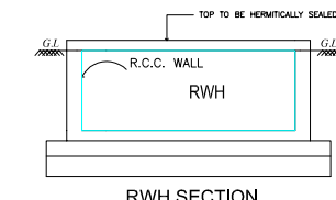
RWH SECTION RWH_CAPACITY_L=5000LTRS
