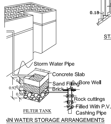
IN WATER STORAGE ARRANGEMENTS
