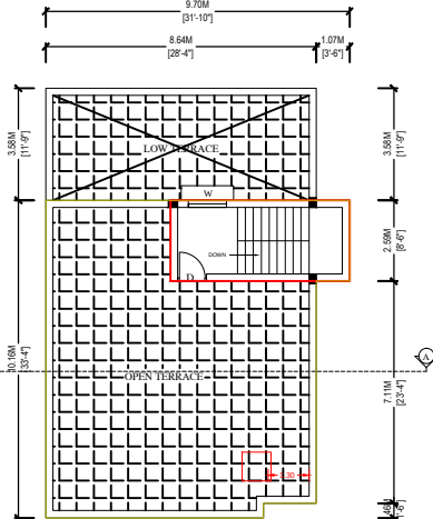
PRO.TERRACE FLOOR PLAN
