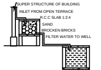
RAINWATER HARVESTING
