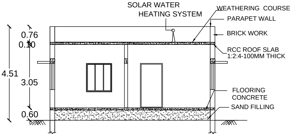
SECTION ON BR
