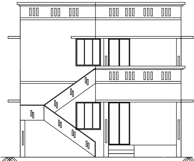
FRONT ELEVATION
