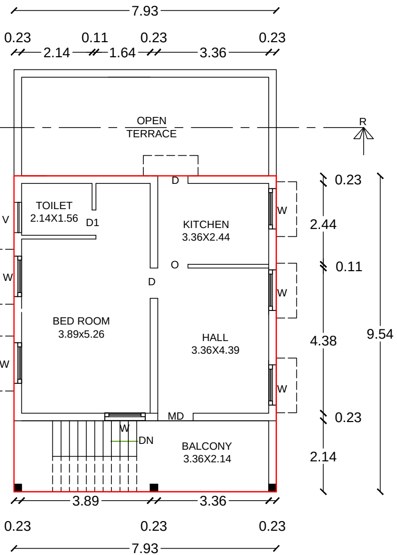
PRO- FISRT FLOOR PLAN
