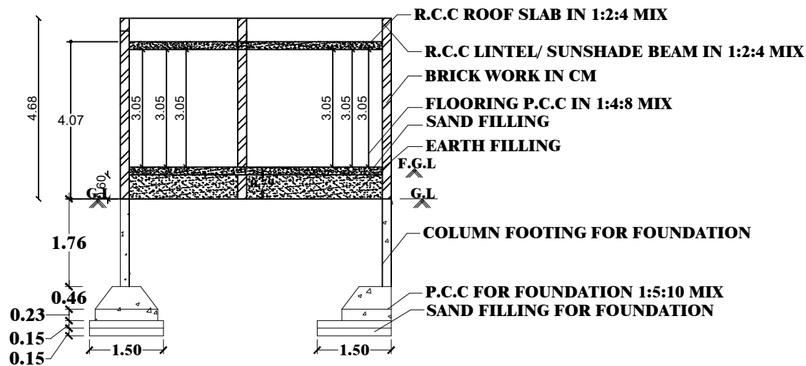
SECTION ON-SD
