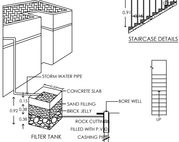
RAIN WATER STORAGE ARRANGEMENTS
