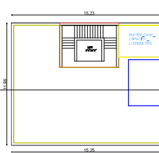
TERRACE FLOOR PLAN
