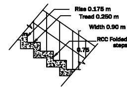
STAIRCASE DETAILS
