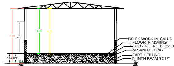
SECTION ON XX
