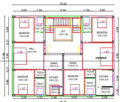
FIRST FLOOR PLAN TYPICAL_FLOOR_PLAN=1,2,3
