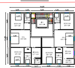
THIRD FLOOR PLAN
