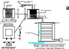
RAIN WATER COLLECTION SYSTEM FROM TERRACE
