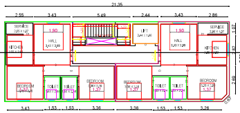
FIRST FLOOR PLAN OR PLAN=1,2,3
