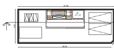
STILT FLOOR PLAN
