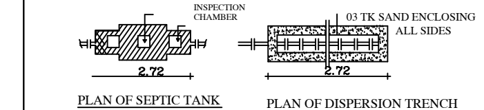
PLAN OF SEPTIC TANK
