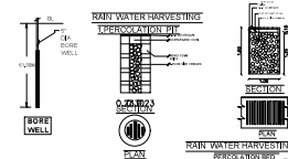
RAIN WATER HARVESTING SYSTEM DETAIL
