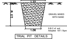
TRIAL PIT DETAILS
